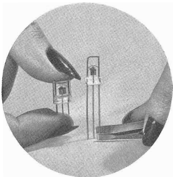
Point-contact type transistors before and after embedding in plastic housing.
